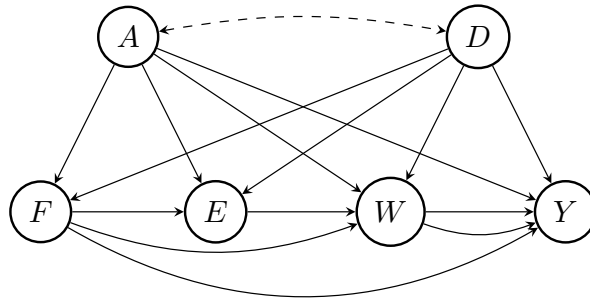
Figure 9: The causal graph for the government-census dataset. D are demographic features, A is gender, F represents marital and family information, E education, W work-related information and Y the salary, which is also the outcome of interest. The bidirected edge between A and D represents that the noise variables U_A and U_D share information.
